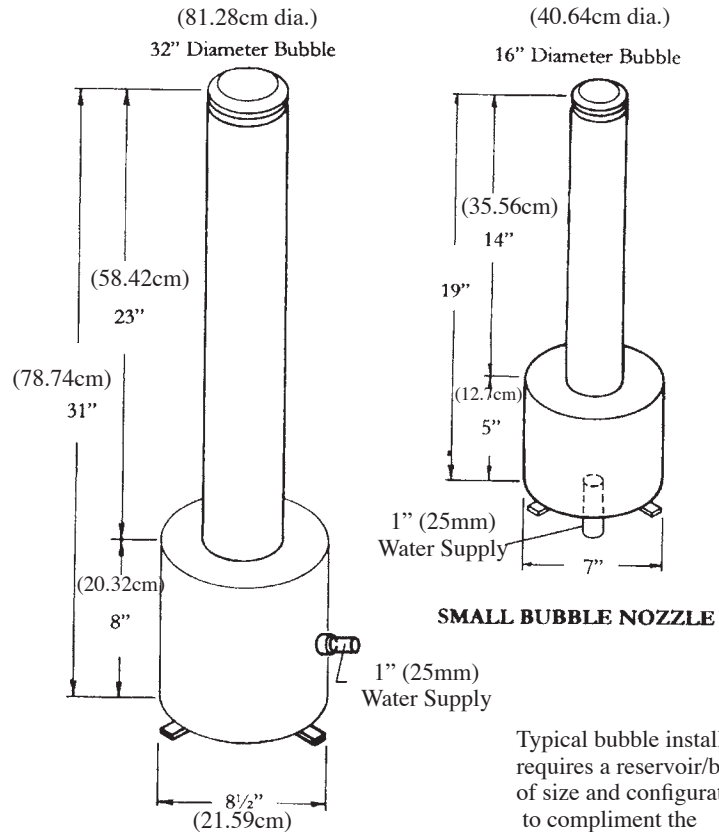
LARGE BUBBLE NOZZLE
