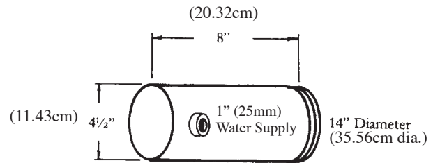
HORIZONTAL BUBBLE NOZZLE
